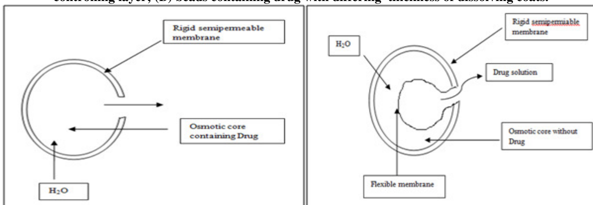
Diagrammatic representation of two types of osmotically controlled system.
